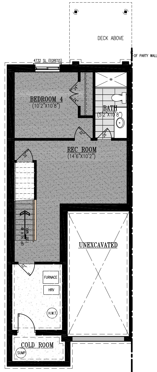
FOUDATION PLAN A1 437 SQ. FT. FINISHED
