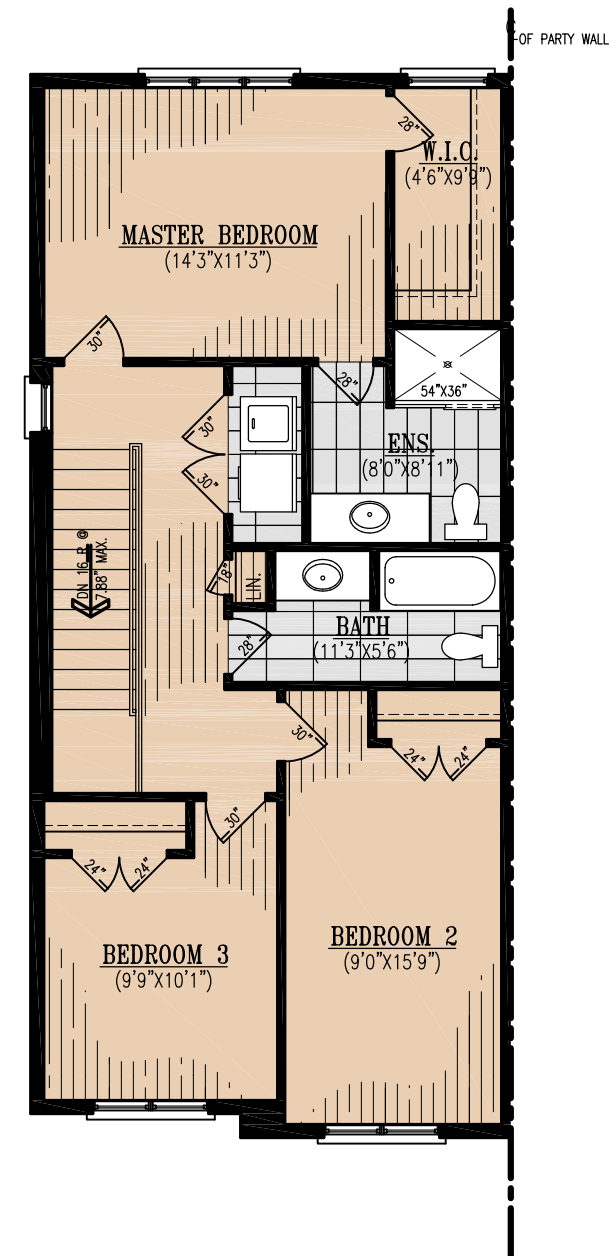
UPPER FLOOR PLAN A1 856 SQ. FT.
