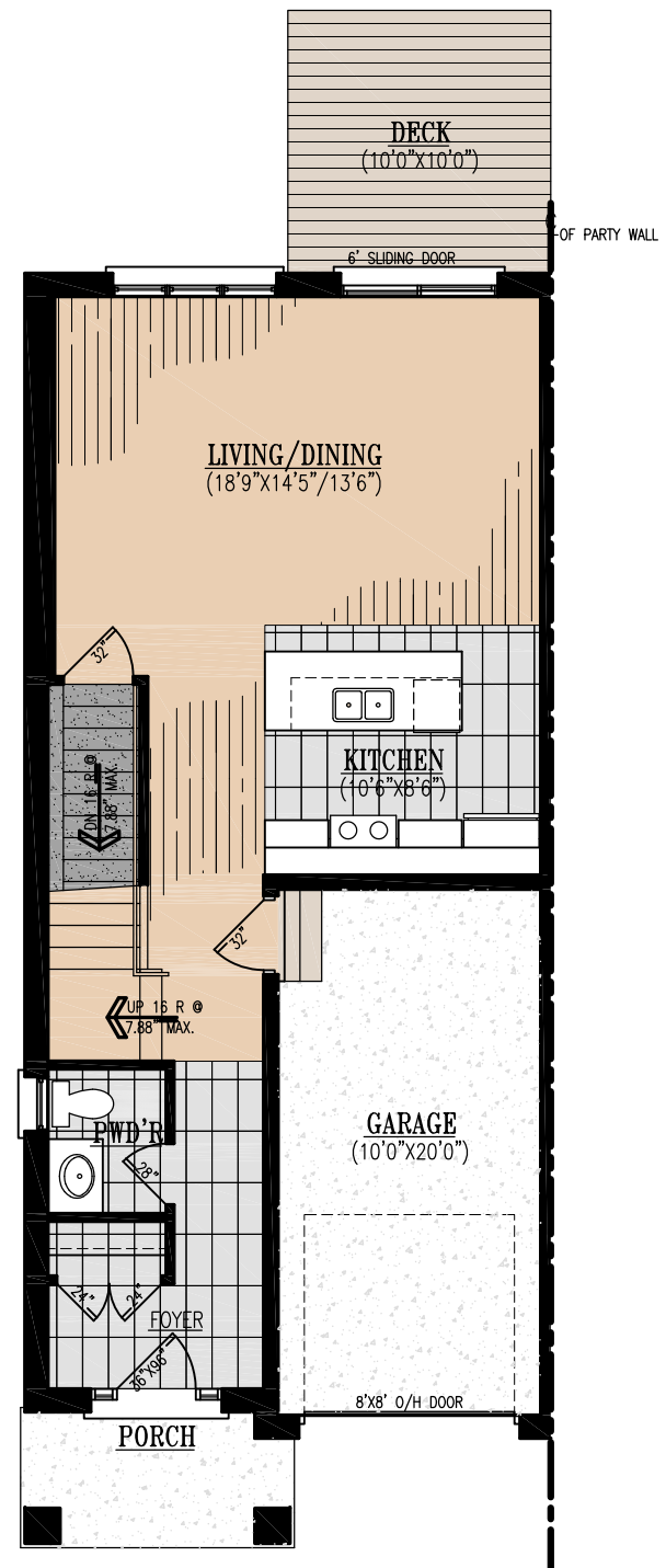
MAIN FLOOR PLAN A1 638 SQ. FT. (1497 SQ.FT. TOTAL)
